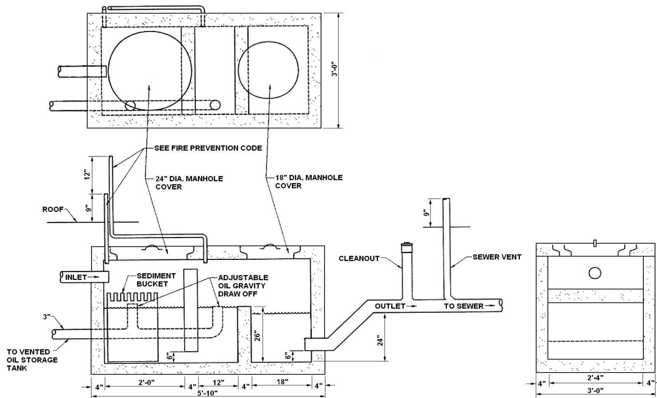
Figure 1005.N.7B—Oil Separator Details
